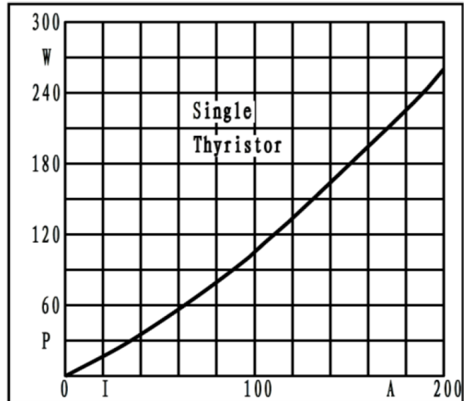
Fig3. Power dissipation
